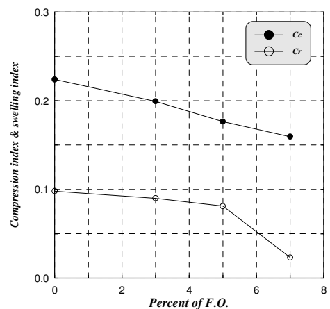
Figure 9 -The relationship of compression index & swelling index with percent of F.O for soil II
