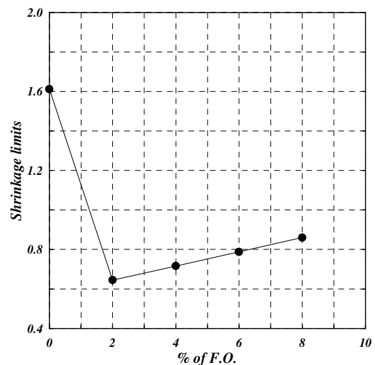
Figure 1 - The relationship between shrinkage limit and percent of fuel oil.
