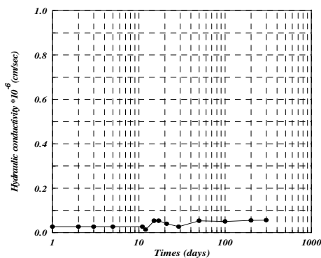
Figure 6 - The hydraulic conductivity for soil I with 8% treatment
