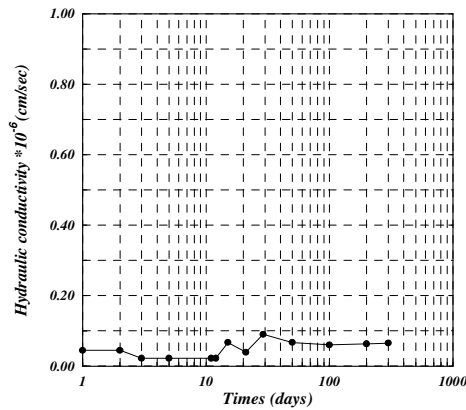
Figure 5 - The hydraulic conductivity for soil I with 6% treatment
