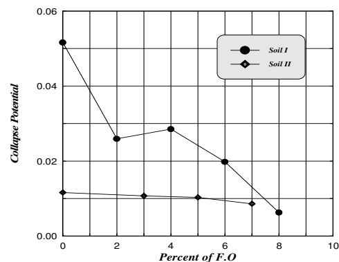
Figure 7 - The relationship between collapse potential and percent of F.O. for Soil I and II
