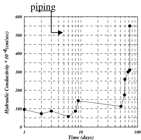
Figure 3 - The hydraulic conductivity for soil I with 2%
