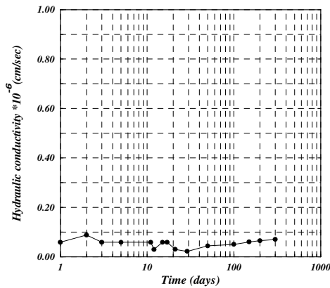
Figure 4 - The hydraulic conductivity for soil I with 4% treatment
