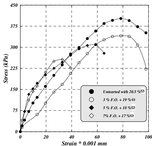
Figure 11 - The relationship between the stress and axial strain of soil II
