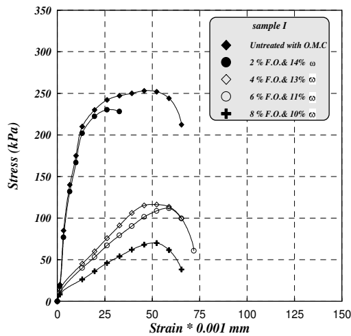
Figure 10 - The relationship between the stress and axial strain of soil I
