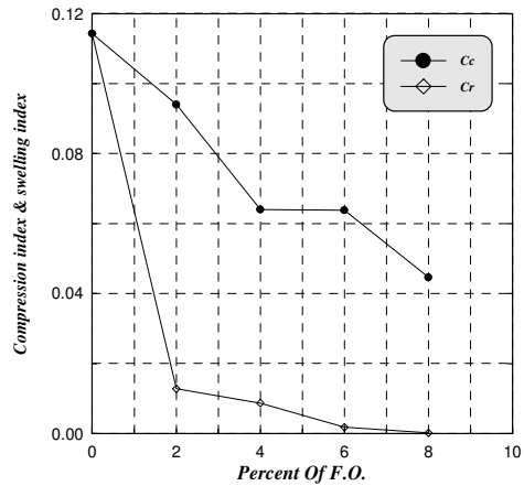
Figure 8 - The relationship of compression index & swelling index with percent of F.O for soil I
