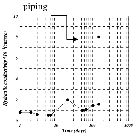
Figure 2 - The hydraulic conductivity for untreated soil
